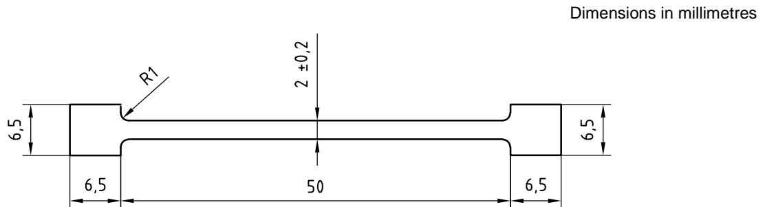
Figure 3 — Narrow test piece
